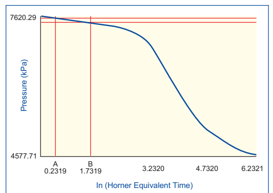
Example of Horner Build-Up Plot
