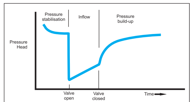
DST Build-up plot
