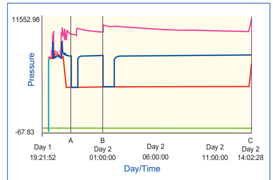
Example Total Plot of Sigra Drill Stem Test (DST)
