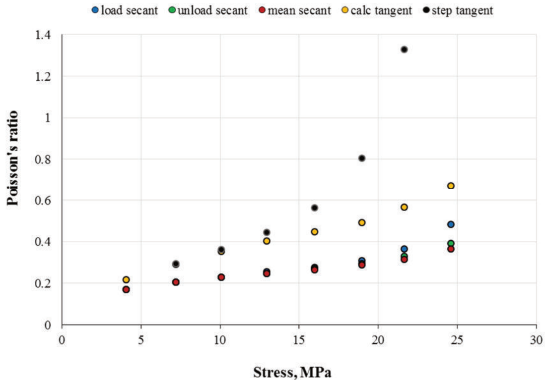
Figure 8 Poisson's ratios calculated by various methods
