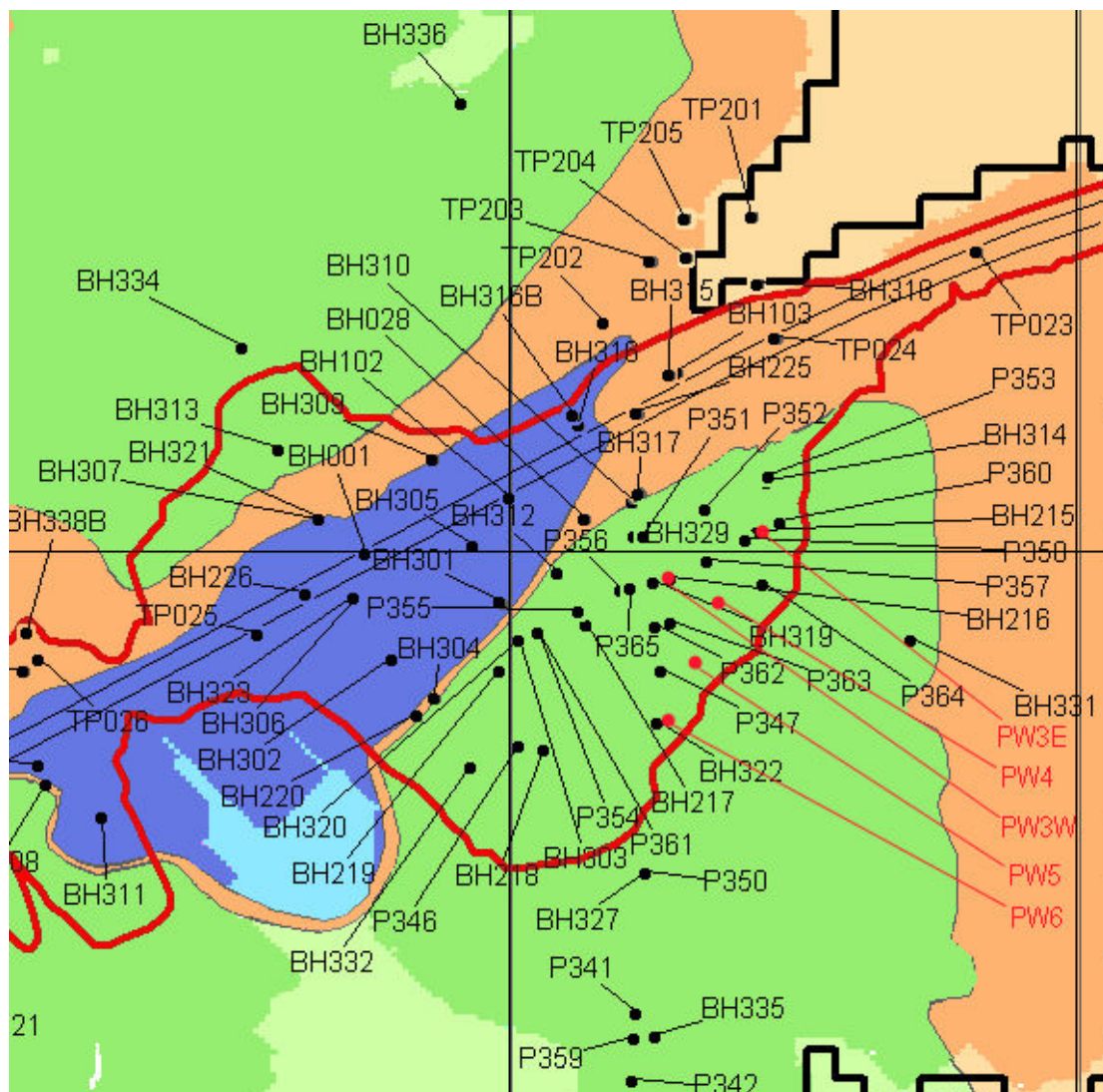
Figure 1 Plan of the area. The area of cut 3 in question is to the south of the roadway and is marked by the cut boundary (in red). The trachyte is shown in green, basalt in blue and sedimentary rocks in orange. Pumping test wells are shown in red. Most other holes contained piezometers
