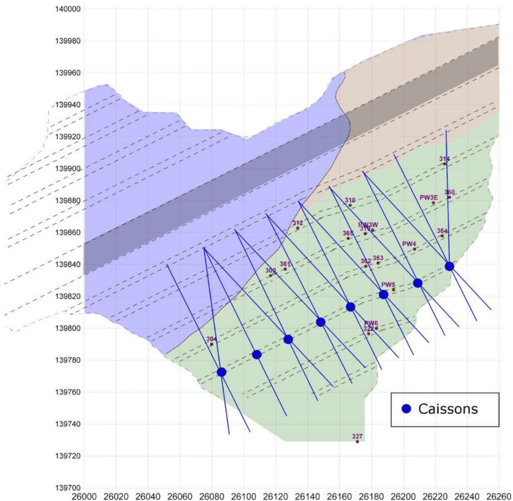
Figure 6 The favoured design using drilled dipping drains that pass through pumped caissons
